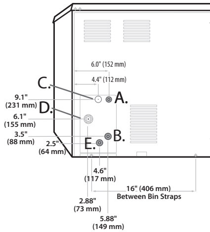
Water Cooled
