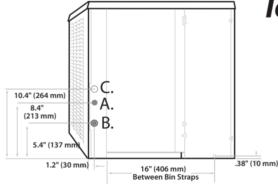
Air Cooled
